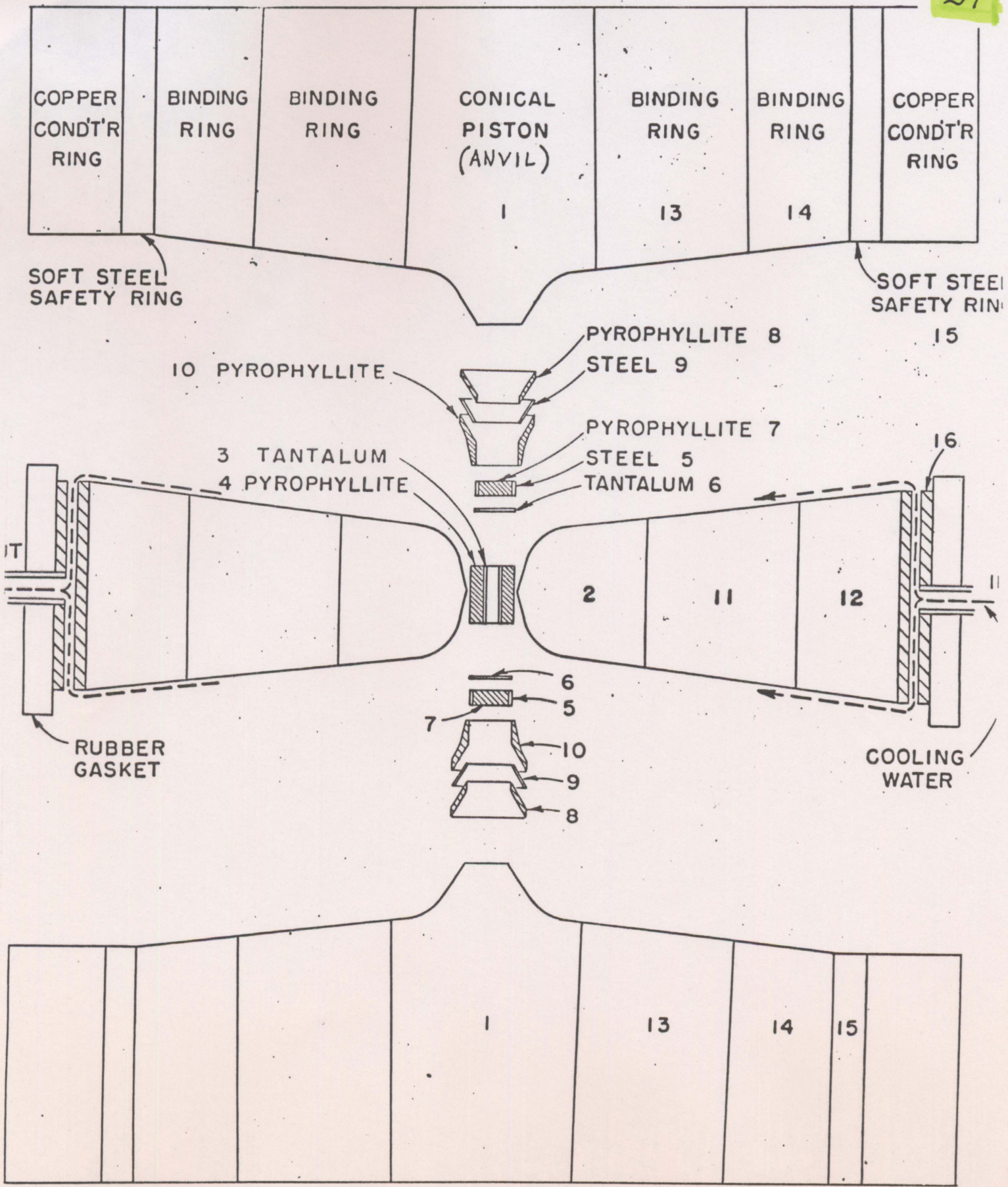
BELT, EXPLODED VIEW
